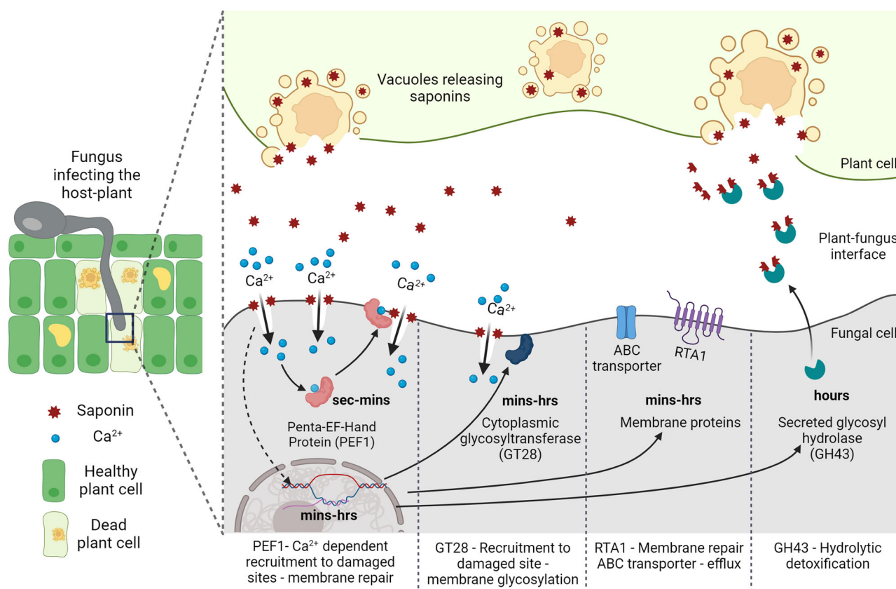
Fig. 8 | Model illustrating the responses of B. cinerea to \alpha -tomatine, both in space and time. The responses start from the moment that \alpha -tomatine is released from the plant vacuoles upon plant cell damage or death inflicted by fungal
