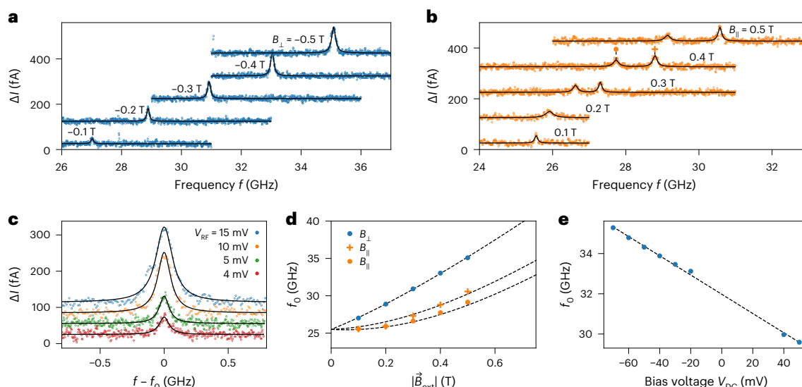
Fig. 2 | ESR spectra of the quantum sensor. a , ESR spectra measured with different B_{\perp} on the bare Ag(111) surface ( V_{DC} = -70 mV, I = 5 pA, V_{RF} = 15 mV). The current difference \Delta I results from the different spin state populations of the quantum sensor and the tunnelling magnetoresistance effect during the ESR frequency sweep. The spectra are shifted vertically by multiples of 100 fA for clarity. Black lines are fits with a Lorentzian function. b , Same as a , but for B_{\parallel} . c , Magnified view of the ESR spectrum at B_{\perp} = -0.5 T for different driving amplitudes V_{RF} ( V_{DC} = -70 mV, I = 10 pA). Fitting a Lorentzian function yields a
