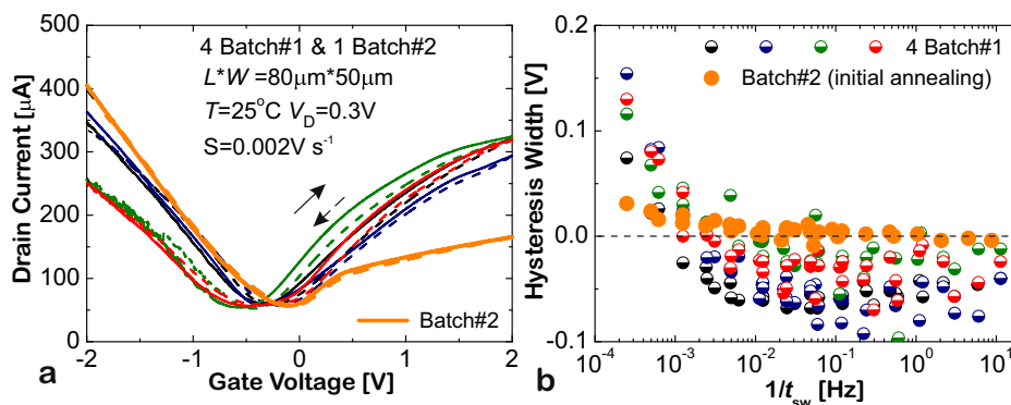
Fig. 4 | Hysteresis dynamics in our GFETs with \text{CaF}_2 . a Double sweep I_D - V_G characteristics of five GFETs with 80 \mu\text{m} \times 50 \mu\text{m} channels measured using ultra-slow sweeps with S = 0.002 \text{ V s}^{-1} . Among these devices, there is one GFET from Batch#2. b The \Delta V_H vs. 1/t_{\text{sw}} dependencies for the same GFETs. Compared to GFETs from Batch#1, the device from Batch#2 has only a small clockwise hysteresis at slow sweeps with no counterclockwise hysteresis at fast sweeps.
