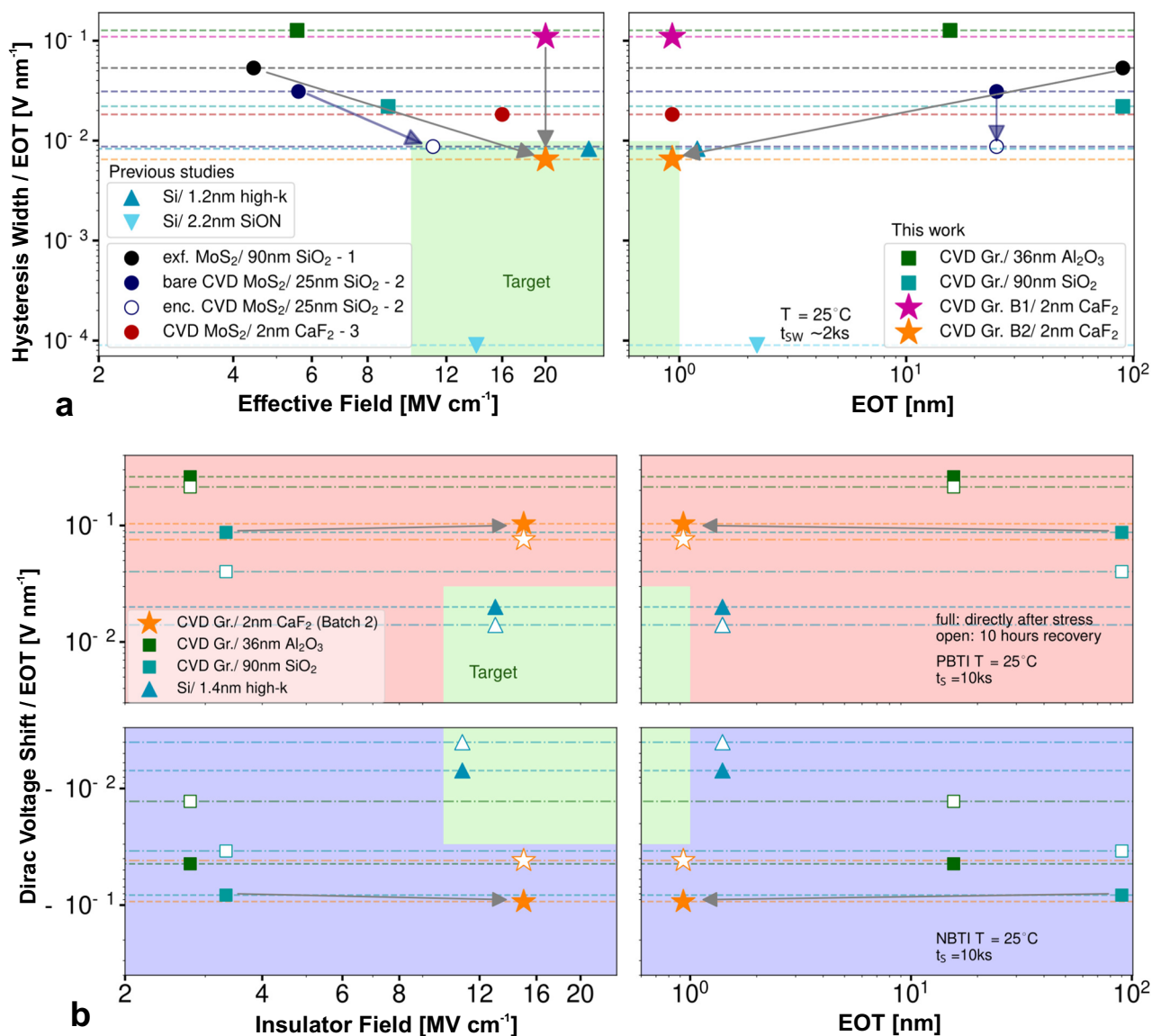
Fig. 8 | Comparison of hysteresis and BTI shifts measured for our GFETs with CaF 2 and other technologies. a Comparison of the normalized hysteresis widths in different back-gated 2D FETs ( 10^{-36} – 2^{-41} – 3^{-22} ) and Si FETs for the sweep time of about 2 ks versus the effective gate field ( V_{G,\text{max}} - V_{G,\text{min}}/d_{\text{ins}} ) (left) and versus EOT (right). For comparing the hysteresis widths on technologies with different gate stacks, the hysteresis widths were normalized by EOT. The measured clockwise hysteresis in our GFETs with CaF 2 is comparable to the normalized hysteresis widths reported in 2D devices, with the hysteresis on our Batch#2 CaF 2 GFETs being the
