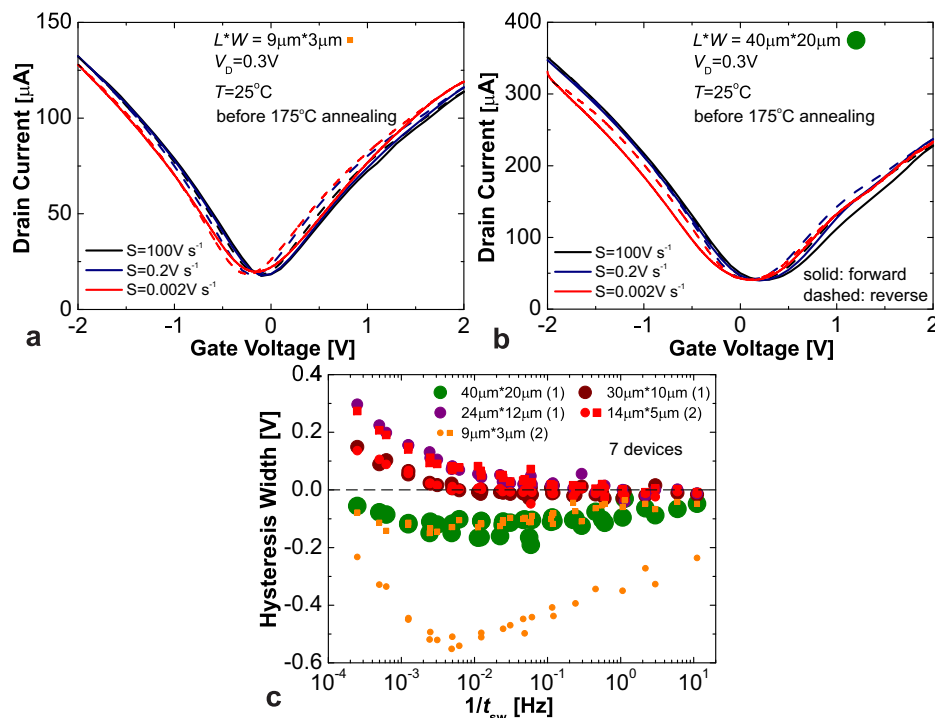
Fig. 5 | Impact of channel dimensions on the hysteresis dynamics. Double sweep I_D - V_G characteristics of GFETs with 9\ \mu\text{m} \times 3\ \mu\text{m} (a) and 40\ \mu\text{m} \times 20\ \mu\text{m} (b) channels measured with different sweep rates. The hysteresis dynamics observed for these two devices are very similar. c The \Delta V_H vs. 1/t_{\text{sw}} dependencies for seven GFETs with different channel dimensions. While there is some variability in the hysteresis dynamics, some devices with different sizes have identical hysteresis and thus this effect appears to be independent of the channel dimensions.
