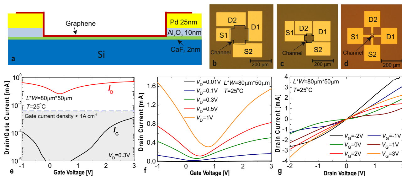
Fig. 1 | Layout and performance of our GFETs with CaF 2 . a Schematic structure of our back-gated GFETs with 2 nm CaF 2 insulators. Optical images of GFETs with L \times W of 160 μm × 100 μm ( b ), 80 μm × 50 μm ( c ) and smaller dimensions from 40 μm × 20 μm to 9 μm × 3 μm ( d ). e The gate leakage current through our thin CaF 2 layers is small compared to the drain current through the GFET channel with a
