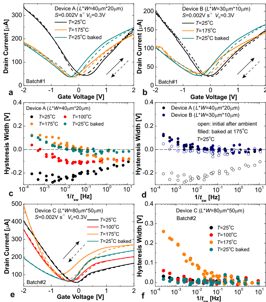
Fig. 6 | Impact of annealing on the hysteresis dynamics. Double sweep I_D - V_G characteristics measured for our Batch#1 GFETs at T = 25^\circ\text{C} , 175^\circ\text{C} and 25^\circ\text{C} after annealing using S = 0.002\text{ V s}^{-1} . Just after 10 min of ambient exposure, Device A (a) exhibited counterclockwise and Device B (b) clockwise hysteresis. c At 100^\circ\text{C} and at 175^\circ\text{C} the counterclockwise hysteresis in Device A is strongly suppressed, and after annealing at 175^\circ\text{C} both devices exhibit similar clockwise hysteresis (d). e, f The corresponding results for a Batch#2 GFET which show no counterclockwise contribution and conventional thermal activation of charge trapping. These GFETs experienced an initial annealing of 2 days at 100^\circ\text{C} and 5 h at 175^\circ\text{C} prior to the first measurement round.
