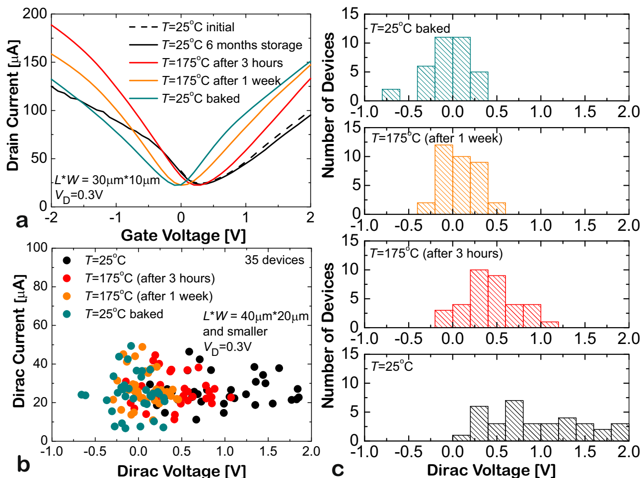
Fig. 3 | Impact of storage and annealing on the performance of our GFETs with \text{CaF}_2 . a Transformation of the I_D - V_G characteristics following 6 months of storage under a moderate vacuum, subsequent annealing at 175 °C and cooling back to 25 °C. b Distribution of I_{\text{Dirac}} vs. V_{\text{Dirac}} for 35 devices at 25 °C, in the beginning and in
