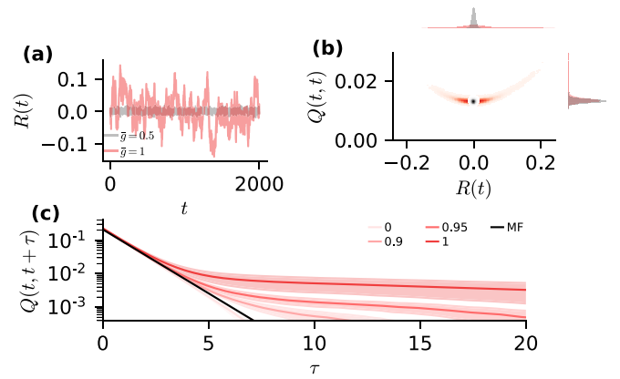
FIG. 1. (a) Population-averaged activity R(t) for \bar{g} = 0.5 (gray) and \bar{g} = 1 (red). (b) Auxiliary fields Q and R , proportional to population-averaged output autocorrelation and activity, respectively, binned for each point in time. (c) Time-lagged, population-averaged, stationary autocorrelation Q(t, t + \tau) simulated for different values of \bar{g} (shades of red) for multiple seeds (shaded background shows the standard deviation) and mean field prediction (black) plotted log-logarithmically. Remaining network parameters: \phi(x) = \text{erf}(\frac{\sqrt{\pi}}{2}x) , N = 1000 , g = 0.5 , and D = 0.1 .
