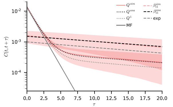
FIG. 3. Time lagged population-averaged autocorrelation Q(t, t + \tau) (3) simulated (red) with standard deviation across seeds (shaded), mean-field theory (gray), fluctuation expansion (12) (gray dotted) and self-consistent solution (25) (black dotted) together with autocorrelation \langle R(t + \tau)R(t) \rangle = \beta_{11}(\tau) of population-averaged activity R (2) (dashed, self-consistent in black, empirical in red, exponential decay with time scale (1 - \bar{g}\langle \phi' \rangle)^{-1} in gray) plotted logarithmically for \bar{g} = 1.0 . Other parameters as in Fig. 1.
