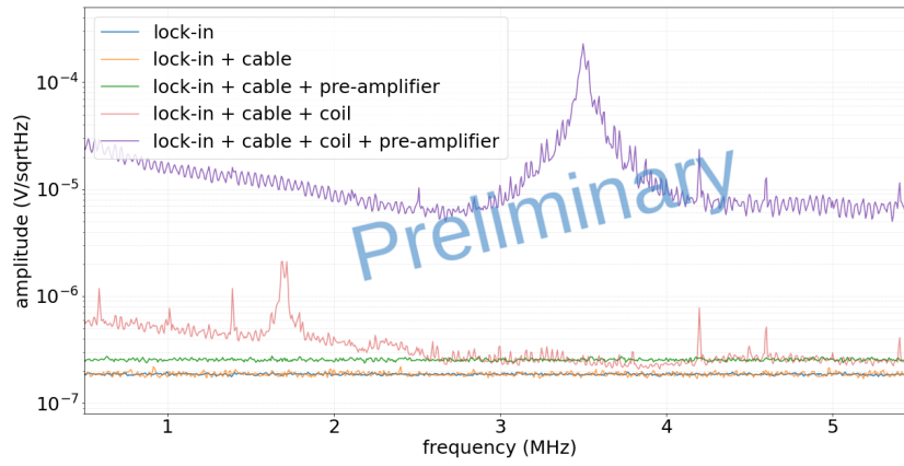
Figure 2: Noise profile of different components at 1V input range.
