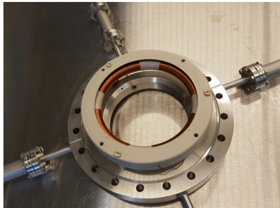
Figure 1: A Rogowski Beam Position Monitor installed inside a vacuum apparatus.
