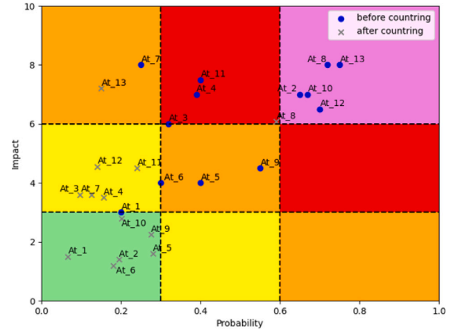
Fig. 16. Illustration of quadrant plot depicting the DSS result to the ADT scenario.
